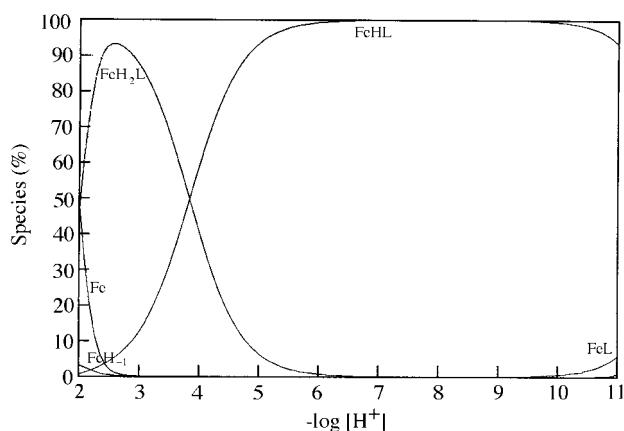
Fig. 5 Species distribution diagram for the system Fe III -TETMAHA as a function of pH ( C_L/C_{Fe} = 10 ; C_{Fe} = 1.99 \times 10^{-4} M).
